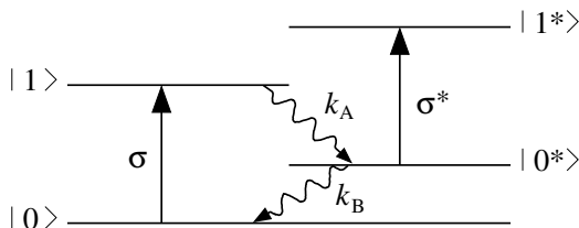
FIGURE 3.5. States and decay scheme used in the model of Section 3.4 to describe the relaxation of the H–Cl stretch vibration. The cross sections for a radiative transition are indicated by \sigma and \sigma^* . The rate of the 1 \rightarrow 0^* relaxation is given by k_A and the rate of the 0^* \rightarrow 0 relaxation is given by k_B .
