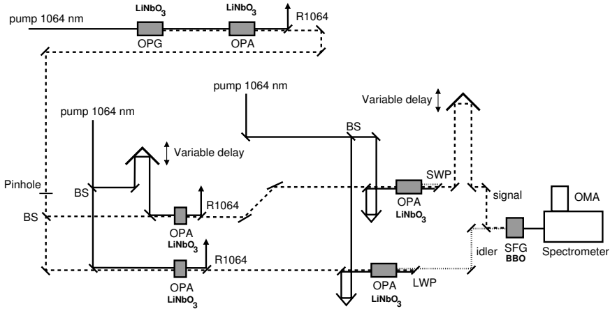
FIGURE 7.3. Experimental set-up for measuring the frequency dependence of the temporal correlation of the parametrically generated light. (Legend: opg: Optical Parametric Generation. opa: Optical Parametric Amplification. bs: beam splitter. swp: Short-wave-pass filter and mirror for 1064 nm. lwp: Long-wave-pass filter and mirror for 1064 nm. sfg: Sum-frequency generation. oma: Optical multichannel analyser. R1064: mirror for 1064 nm.).
