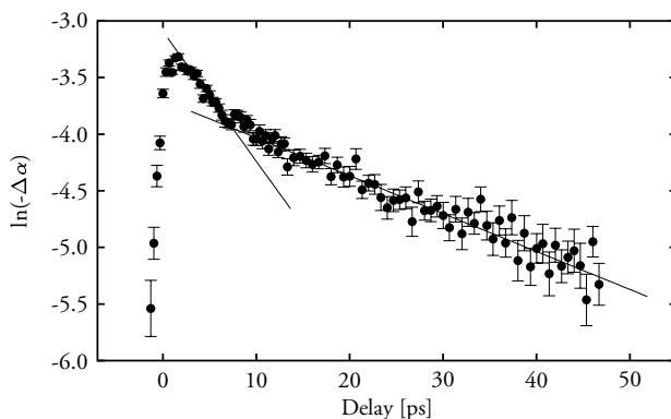
FIGURE 6.3. Pump-probe delay scan of methanol in \text{CCl}_4 at a frequency of 1037\text{ cm}^{-1} ( \lambda=9.64\text{ }\mu\text{m} ), T=43^\circ\text{C} . The solid lines are guides to the eye and illustrate that the bleaching signal exhibits a bi-exponential decay.
